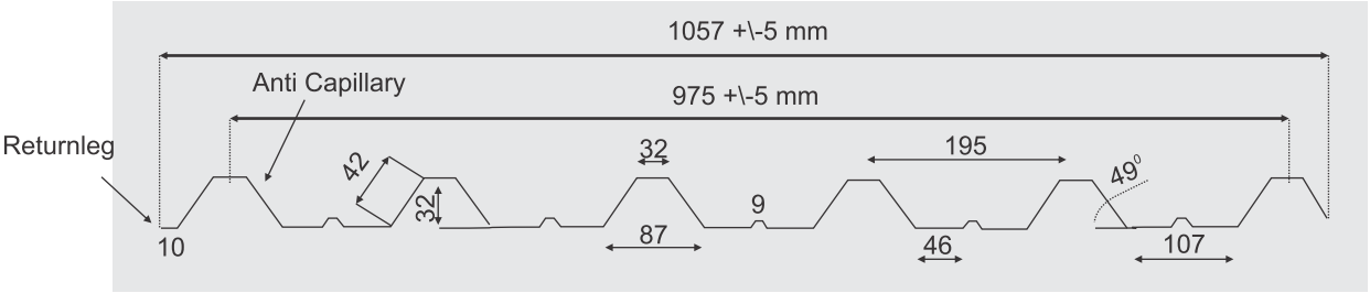
DRAWING
